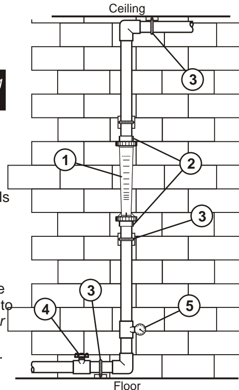
F-452 Meter Installation
