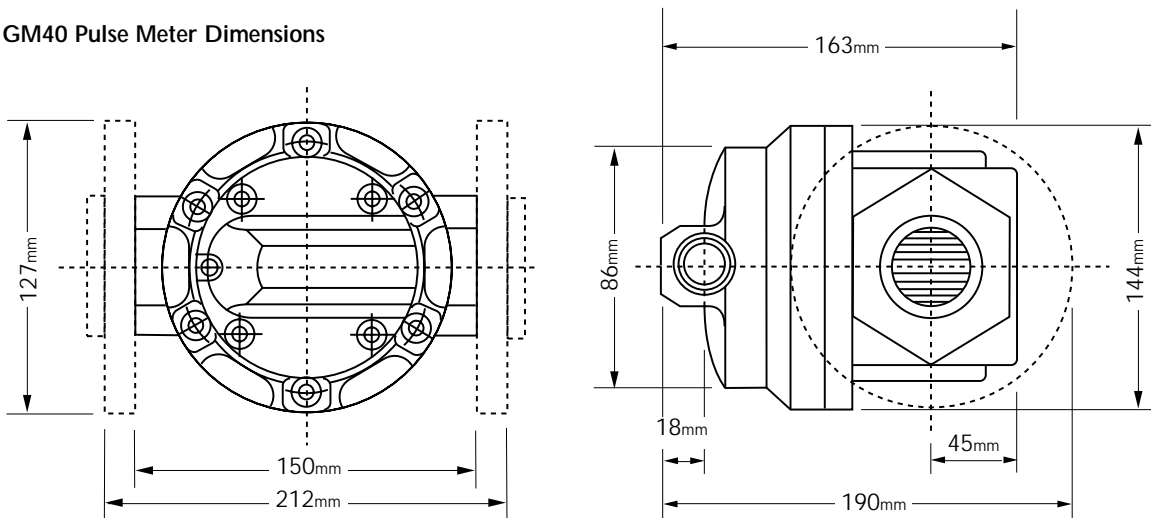
GM40 Pulse Meter with Standard LC Display
