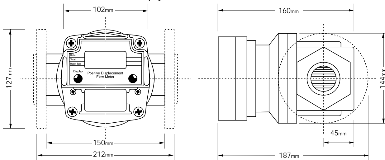
GM40 Pulse Meter with Standard LC Display
