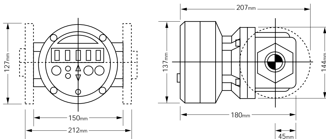
GM40 Pulse Meter with Deluxe LC Display
